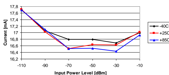
1.2 kBaud GFSK
